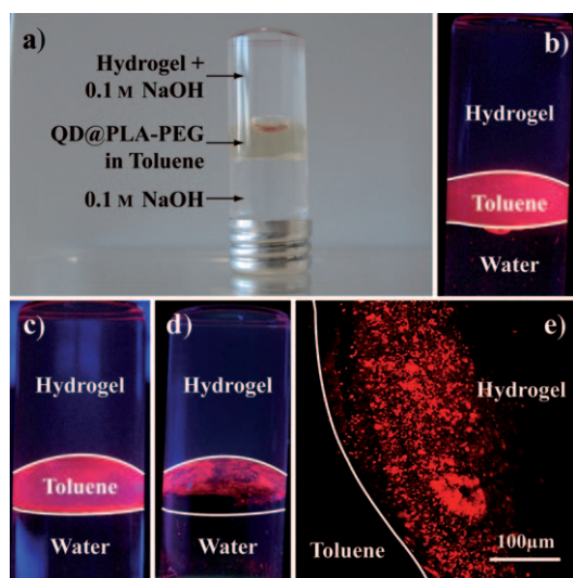
Figure 4. Transfer of CdSe@ZnS@PLA/PEG QDs from the organic phase to the aqueous phase in a triphasic system heated at 40 °C. a,b) Optical images of the initial triphasic systems recorded under sunlight (a) and a UV lamp (b). c,d) UV optical images of the triphasic system (c) and the hydrogel phase (d) washed by toluene and water several times to remove the excess of QDs after 2 days of incubation at 40 °C with gentle shaking. e) CLSM cross-section image of the hydrogel phase from (d), used to determine the QDs penetration depth. The water/toluene and the hydrogel/toluene interfaces are indicated by white lines.
